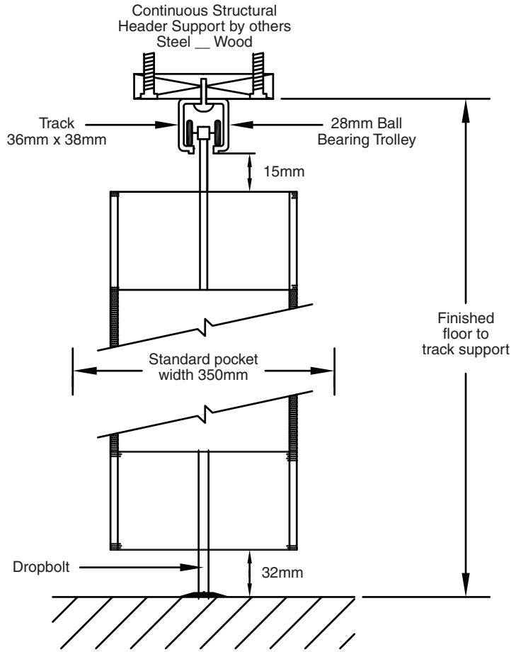
VERTICAL SECTION
